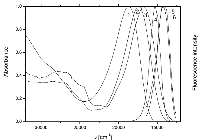
Figure 1. Normalized absorption spectra of compound 2e (curve 1); 4e (curve 2) and 4a (curve 3) and corrected fluorescence spectra of compound 2e (curve 4); 4e (curve 5) and 4a (curve 6) in ethanol (concentration 1 \times 10^{-5} \text{ L mol}^{-1} ) at room temperature.
