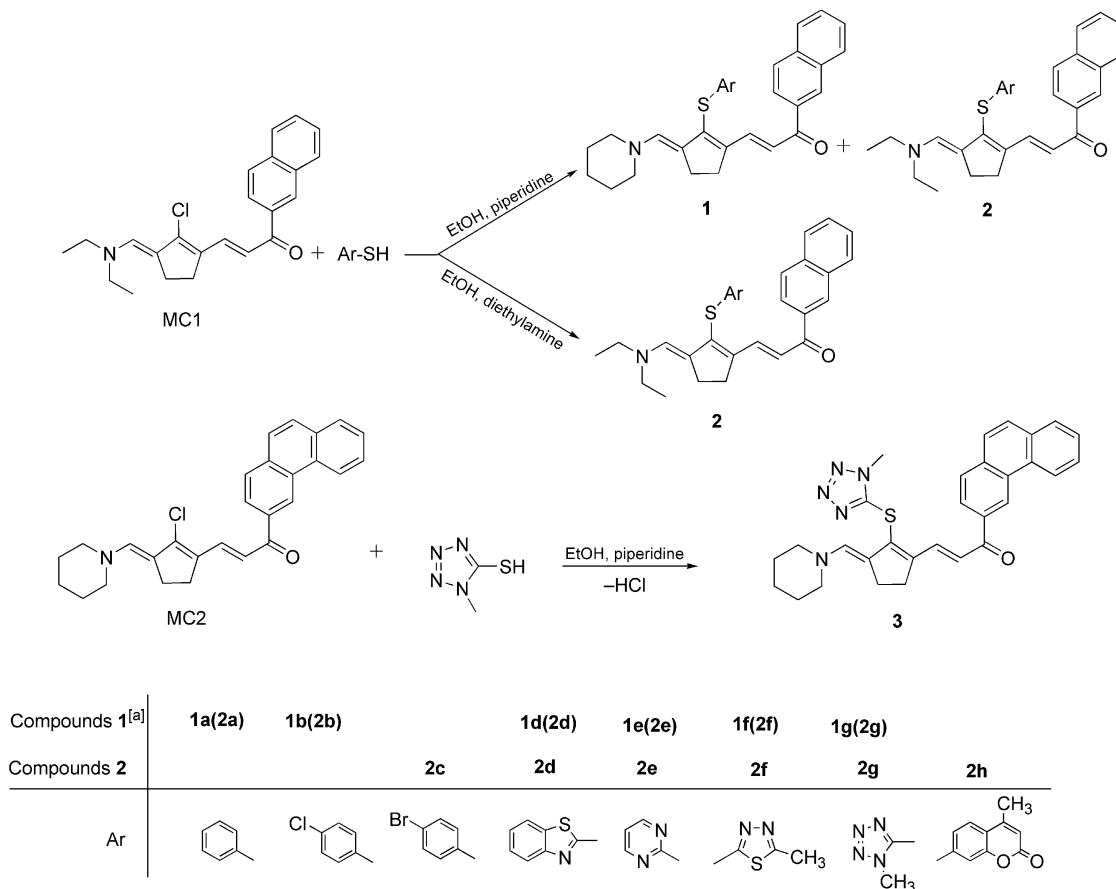
Scheme 1. Synthesis of ramified merocyanine dyes using -SH nucleophiles.
